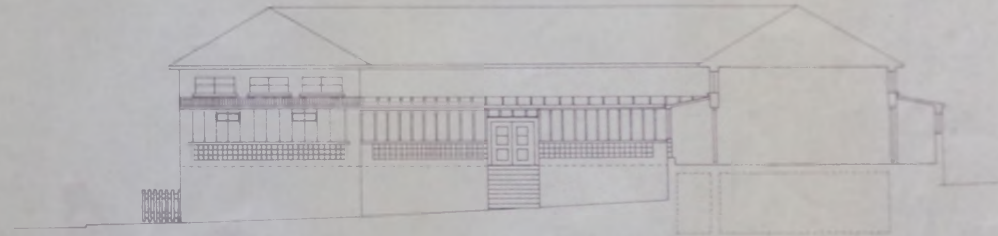
Section/Elevation Thro' Courtyard
