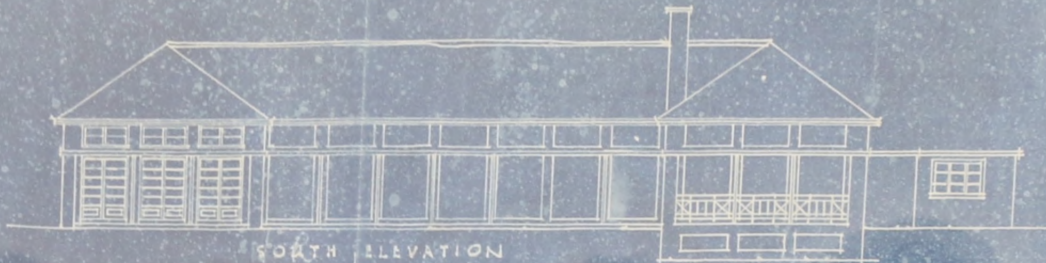
SOUTH ELEVATION
