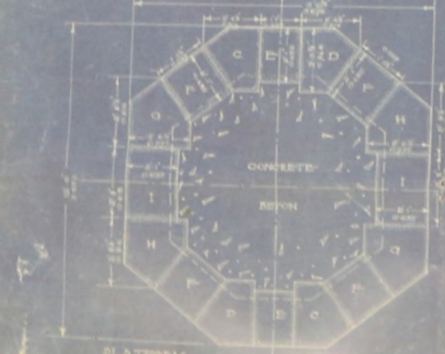
PLATFORM DERNIERE ASSISE
