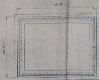
FOUNDATION PLAN
