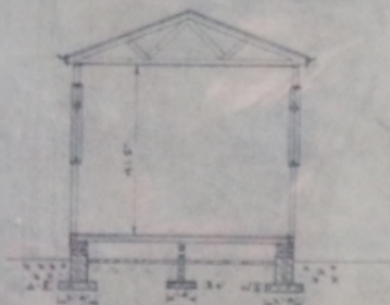
CROSS SECTION X-X
